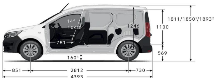
Dimensions (mm)
